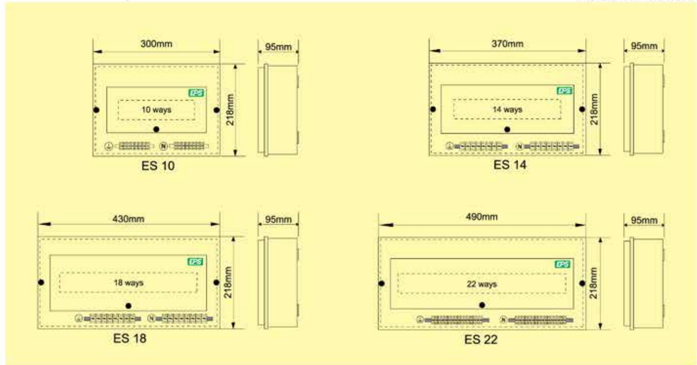
Layout & Dimensions
