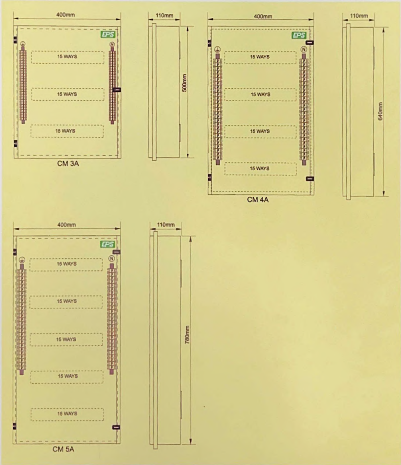
Layout & Dimensions
