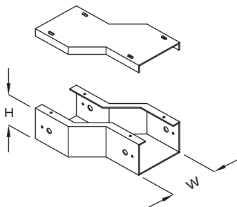
45° Horizontal Offset with Cover (left) Type: UL/TG/A-12
