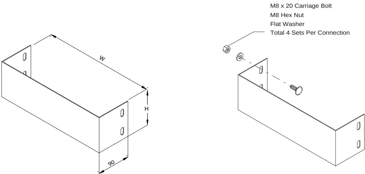
End Plate and Fixture
