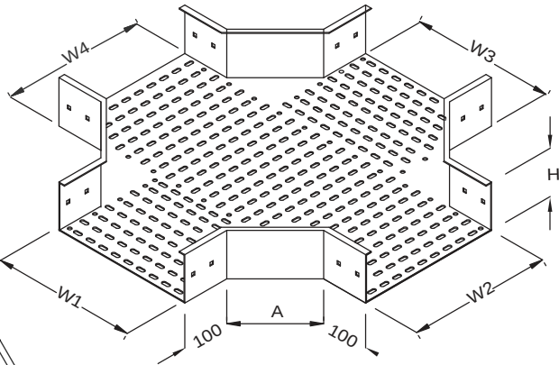
Angular Cross Type: UL/TT/AT or UL/TC/AT-6
