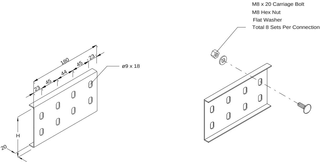
Splice Plate and Fixture
