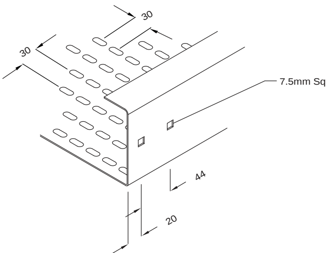
CONNECTION SLOT DETAIL
