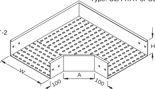
90° Angular Elbow Type: UL/TT/AT or UL/TC/AT-3
