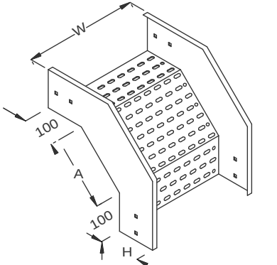
90° Angular External Riser Type: UL/TT/AT or UL/TC/AT-2
